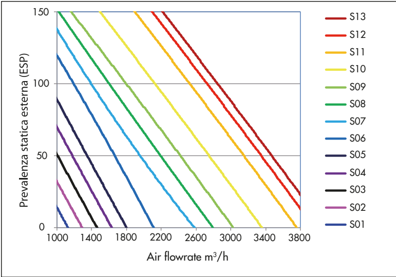
ADG ECO 160PH - static pressure curves
