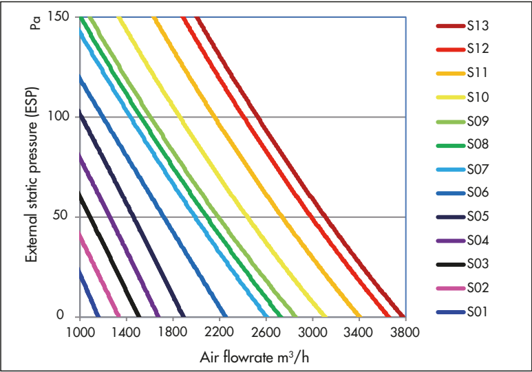
ADG ECO 140PH - static pressure curves
